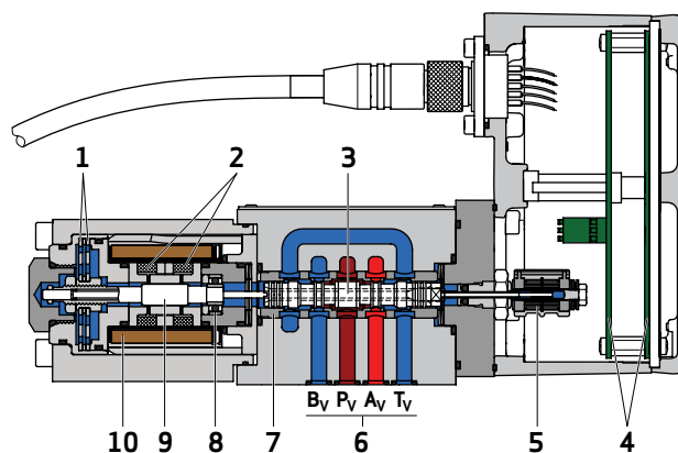
D633 Pilot Valve with Closed-Loop Position Control
